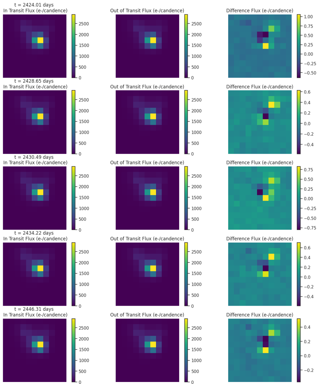
Fig 6. Difference images for target TIC 224290280 for each transit like event. Left: mean in-transit flux(left). Middle: mean out-of-transit flux. Right: difference between the mean out-of-transit and mean in-transit flux. Ensure that the change in brightness occurs on target.
