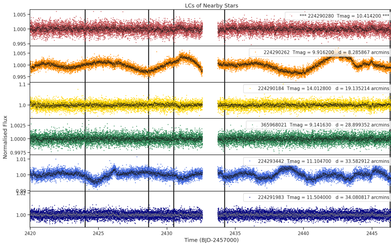
Fig 8. Lightcurves of the five closest stars to target 224290280 (top panel). The distances to the target star and the TESS magnitudes are shown for each star. Only ever shown for one sector.
