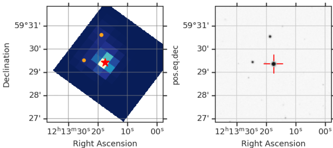
Fig 7. The locations of nearby GAIA DR2 stars with a magnitude difference less than 5 (orange circle) within the TESS Cut Out around TIC 224290280 (red star). Only shown for one sector. Right: SDSS image of the surrounding field.
