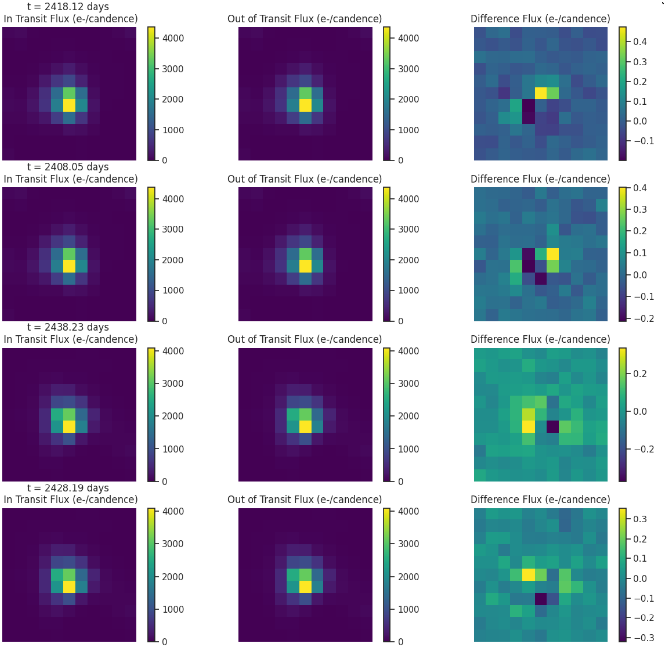
Fig 6. Difference images for target TIC 230023734 for each transit like event. Left: mean in-transit flux(left). Middle: mean out-of-transit flux. Right: difference between the mean out-of-transit and mean in-transit flux. Ensure that the change in brightness occurs on target.
