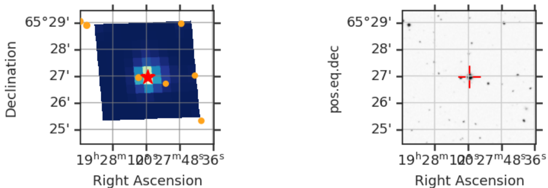
Fig 7. The locations of nearby GAIA DR2 stars with a magnitude difference less than 5 (orange circle) within the Tess Cut Out around TIC 230023734 (red star). Only shown for one sector. Right: SDSS image of the surrounding field.
