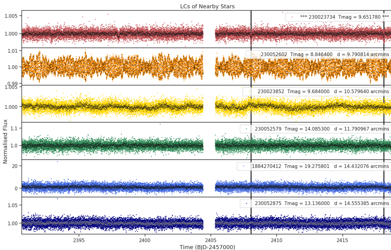
Fig 8. Lightcurves of the five closest stars to target 230023734 (top pannel). The distances to the target star and the TESS magnitudes are shown for each star. Only ever shown for one sector.
