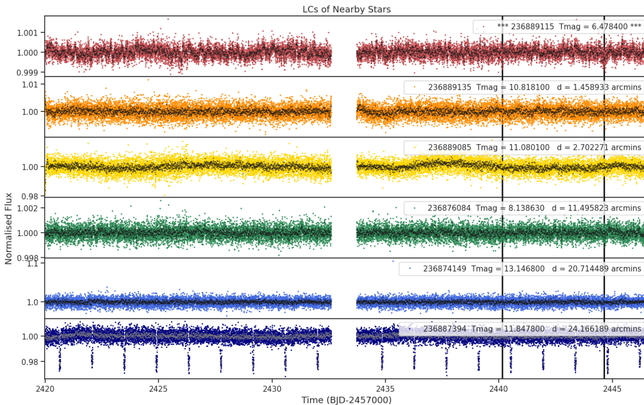
Fig 8. Lightcurves of the five closest stars to target 236889115 (top panel). The distances to the target star and the TESS magnitudes are shown for each star. Only ever shown for one sector.
