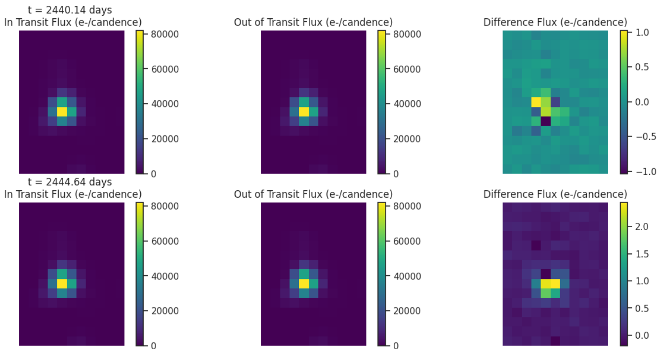
Fig 6. Difference images for target TIC 236889115 for each transit like event. Left: mean in-transit flux(left). Middle: mean out-of-transit flux. Right: difference between the mean out-of-transit and mean in-transit flux. Ensure that the change in brightness occurs on target.
