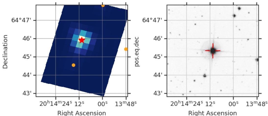
Fig 7. The locations of nearby GAIA DR2 stars with a magnitude difference less than 5 (orange circle) within the Tess Cut Out around TIC 236889115 (red star). Only shown for one sector. Right: SDSS image of the surrounding field.
