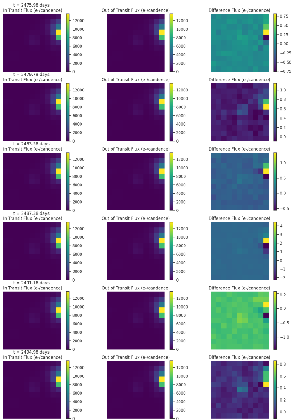
Fig 6. Difference images for target TIC 284326455 for each transit like event. Left: mean in-transit flux(left). Middle: mean out-of-transit flux. Right: difference between the mean out-of-transit and mean in-transit flux. Ensure that the change in brightness occurs on target.
