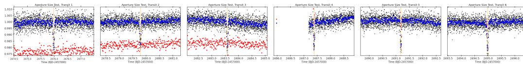
Fig 4. The lightcurve around the time of each transit-like event extracted with the SPOC pipeline defined aperture (binned:blue, uninned:grey) and the with an aperture that is 40 per cent smaller (red). The flux is extracted from the target pixel files (TPFs) and has not been detrended or corrected for systematics. The vertical orange line indicates the time of the transit-like event.
