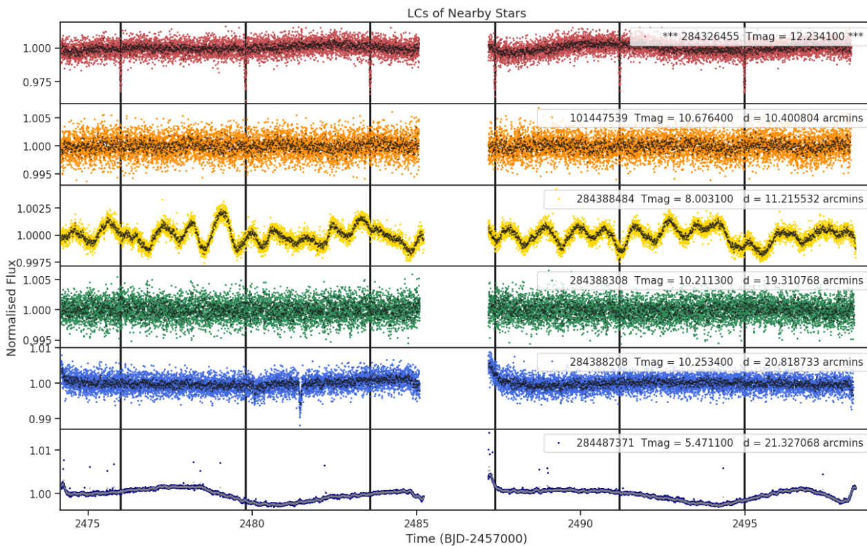
Fig 8. Lightcurves of the five closest stars to target 284326455 (top panel). The distances to the target star and the TESS magnitudes are shown for each star. Only ever shown for one sector.
