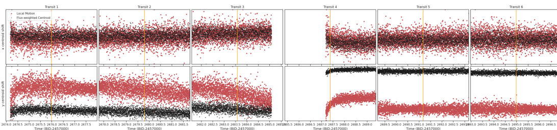
Fig 3. The x and y centroid positions around the time of each transit-like event. The black points shows the CCD column and row position of the target's flux-weighted centroid. The red shows the CCD column and row local motion differential velocity (DVA), pointing drift, and thermal effects. The vertical orange line indicates the time of the transit-like event
