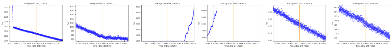
Fig 2. Background flux vs. time around the time of each transit-like event. The vertical orange line indicates the time of the transit-like event.
