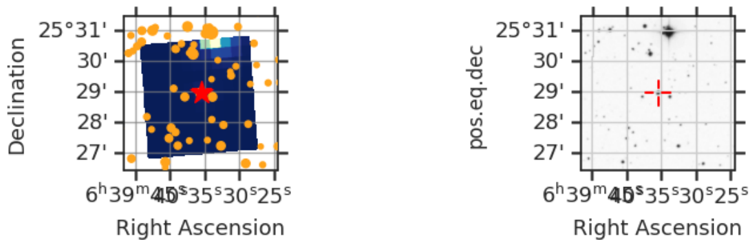
Fig 7. The locations of nearby GAIA DR2 stars with a magnitude difference less than 5 (orange circle) within the Tess Cut Out around TIC 284326455 (red star). Only shown for one sector. Right: SDSS image of the surrounding field.
