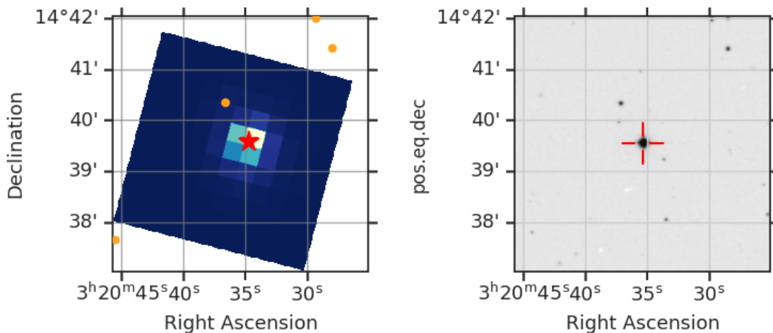
Fig 7. The locations of nearby GAIA DR2 stars with a magnitude difference less than 5 (orange circle) within the TESS Cut Out around TIC 303368830 (red star). Only shown for one sector. Right: SDSS image of the surrounding field.
