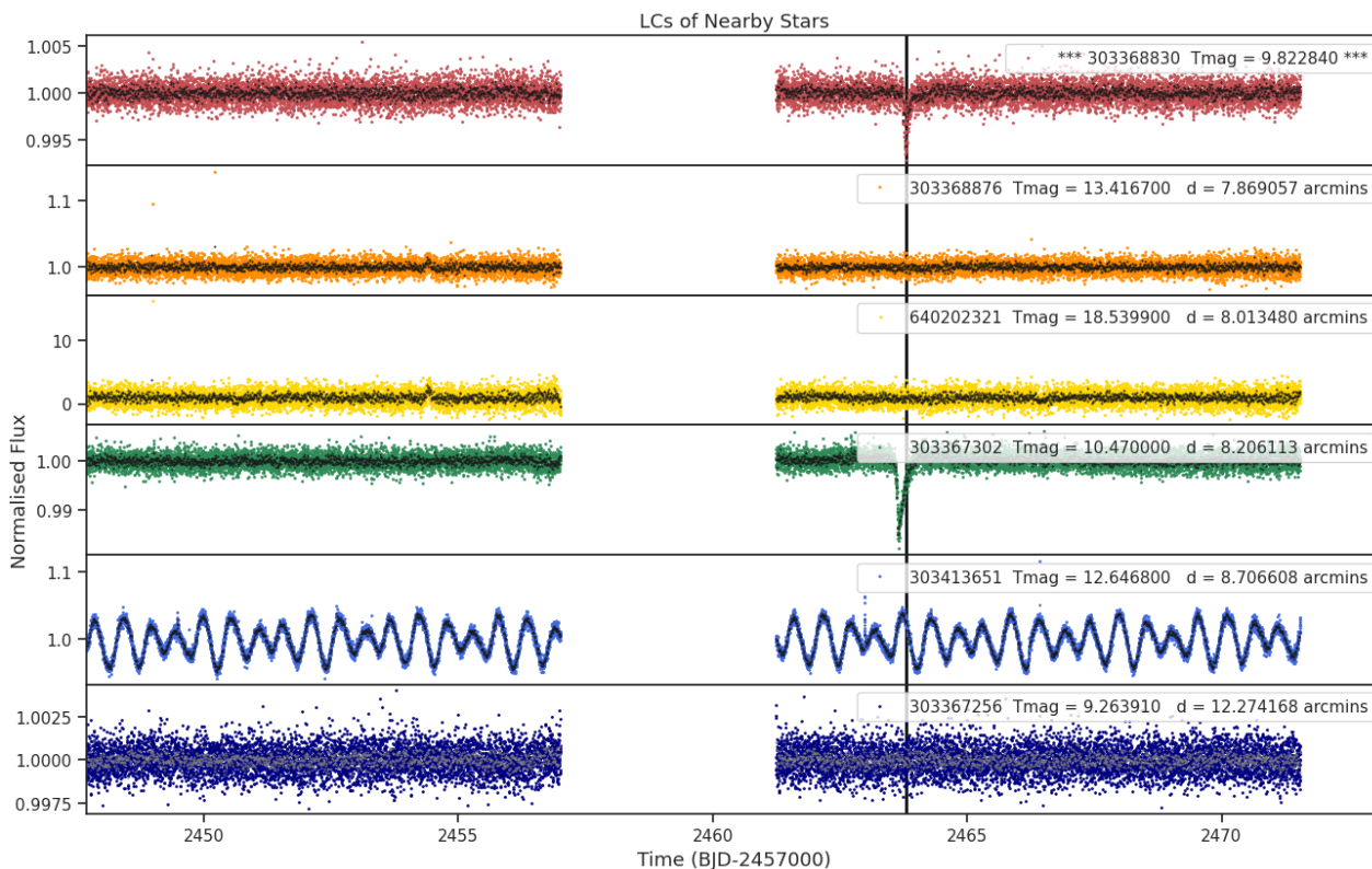
Fig 8. Lightcurves of the five closest stars to target 303368830 (top panel). The distances to the target star and the TESS magnitudes are shown for each star. Only ever shown for one sector.
