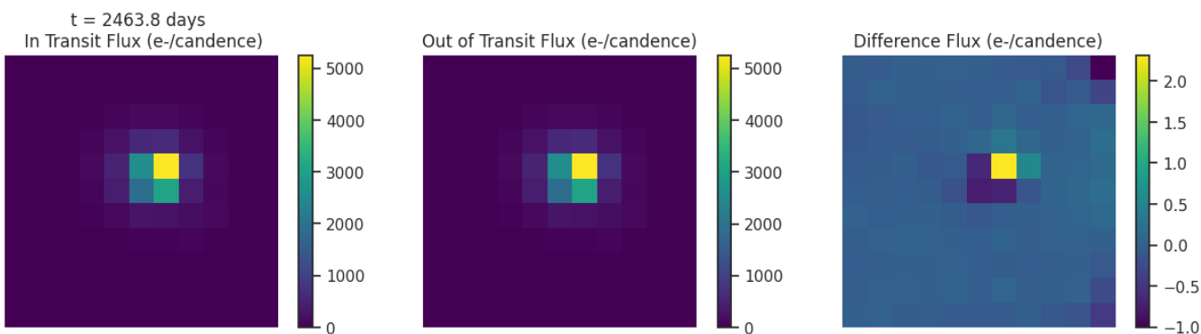
Fig 6. Difference images for target TIC 303368830 for each transit like event. Left: mean in-transit flux(left). Middle: mean out-of-transit flux. Right: difference between the mean out-of-transit and mean in-transit flux. Ensure that the change in brightness occurs on target.
