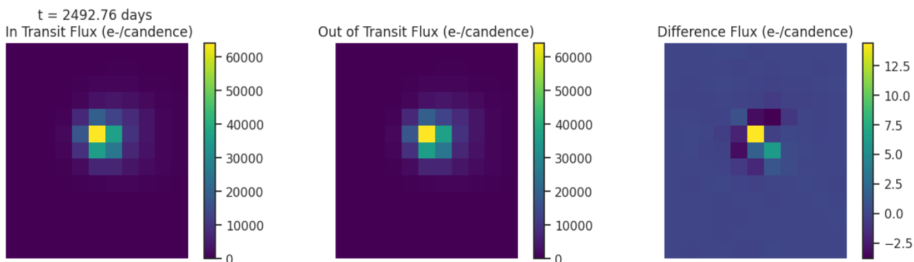
Fig 6. Difference images for target TIC 306216985 for each transit like event. Left: mean in-transit flux(left). Middle: mean out-of-transit flux. Right: difference between the mean out-of-transit and mean in-transit flux. Ensure that the change in brightness occurs on target.
