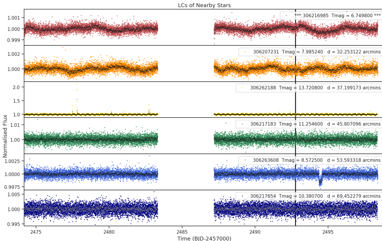
Fig 8. Lightcurves of the five closest stars to target 306216985 (top panel). The distances to the target star and the TESS magnitudes are shown for each star. Only ever shown for one sector.
