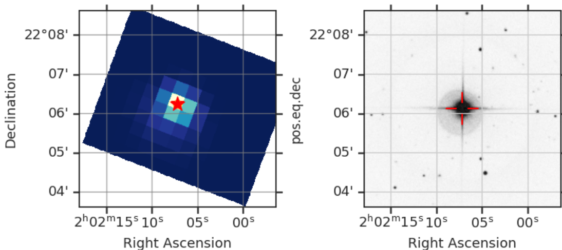
Fig 7. The locations of nearby GAIA DR2 stars with a magnitude difference less than 5 (orange circle) within the TESS Cut Out around TIC 306216985 (red star). Only shown for one sector. Right: SDSS image of the surrounding field.
