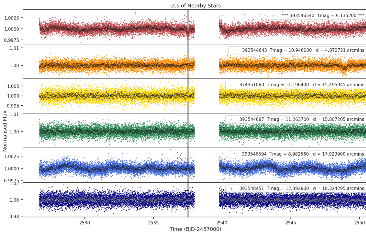
Fig 8. Lightcurves of the five closest stars to target 393546540 (top panel). The distances to the target star and the TESS magnitudes are shown for each star. Only ever shown for one sector.
