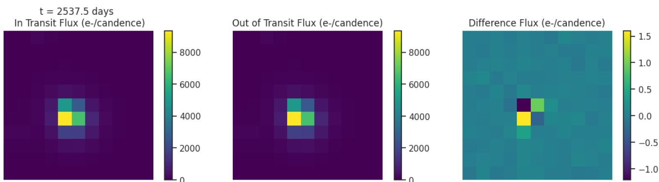
Fig 6. Difference images for target TIC 393546540 for each transit like event. Left: mean in-transit flux(left). Middle: mean out-of-transit flux. Right: difference between the mean out-of-transit and mean in-transit flux. Ensure that the change in brightness occurs on target.
