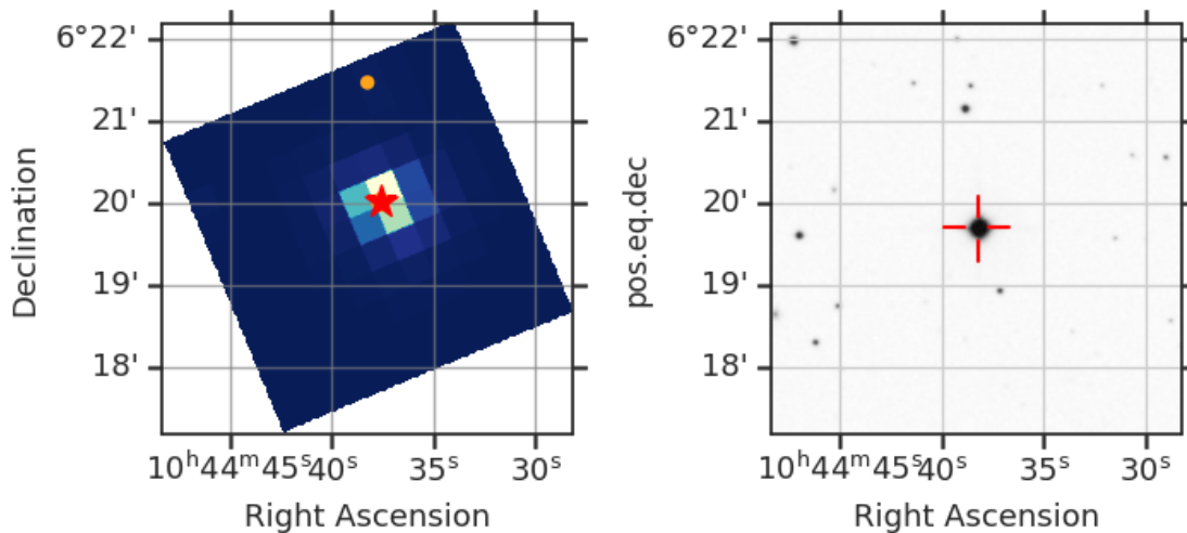
Fig 7. The locations of nearby GAIA DR2 stars with a magnitude difference less than 5 (orange circle) within the TESS Cut Out around TIC 393546540 (red star). Only shown for one sector. Right: SDSS image of the surrounding field.
