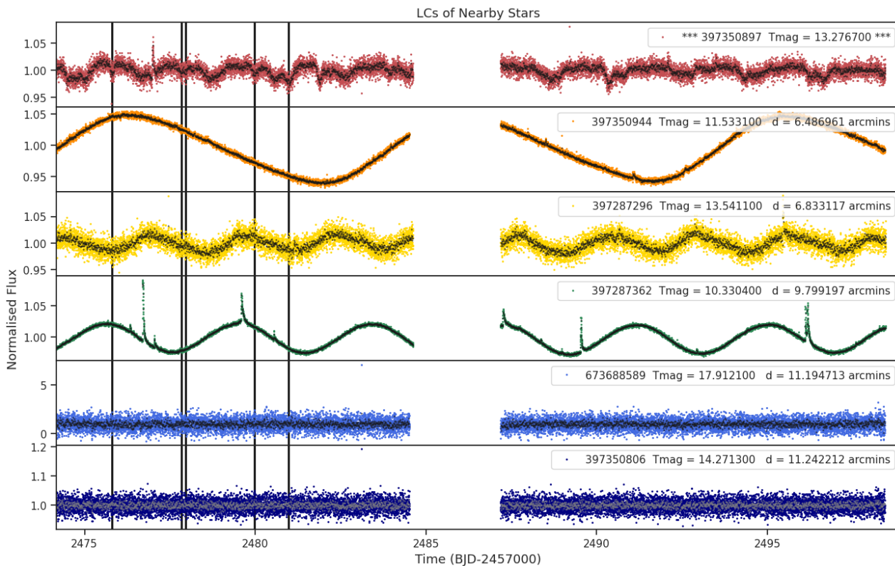
Fig 8. Lightcurves of the five closest stars to target 397350897 (top panel). The distances to the target star and the TESS magnitudes are shown for each star. Only ever shown for one sector.
