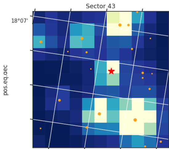
Fig 7. The locations of nearby GAIA DR2 stars with a magnitude difference less than 5 (orange circle) within the Tess Cut Out around TIC 397350897 (red star). Only shown for one sector. Right: SDSS image of the surrounding field.
