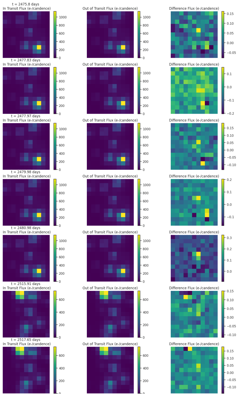
Fig 6. Difference images for target TIC 397350897 for each transit like event. Left: mean in-transit flux(left). Middle: mean out-of-transit flux. Right: difference between the mean out-of-transit and mean in-transit flux. Ensure that the change in brightness occurs on target.
