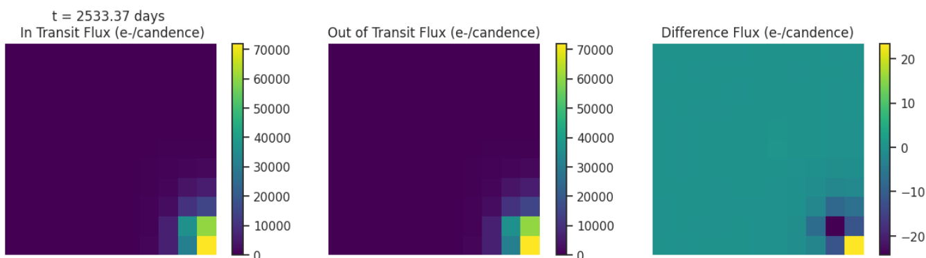
Fig 6. Difference images for target TIC 443616612 for each transit like event. Left: mean in-transit flux(left). Middle: mean out-of-transit flux. Right: difference between the mean out-of-transit and mean in-transit flux. Ensure that the change in brightness occurs on target.
