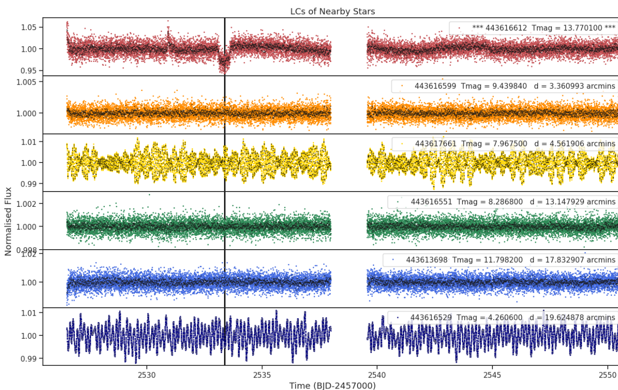
Fig 8. Lightcurves of the five closest stars to target 443616612 (top panel). The distances to the target star and the TESS magnitudes are shown for each star. Only ever shown for one sector.
