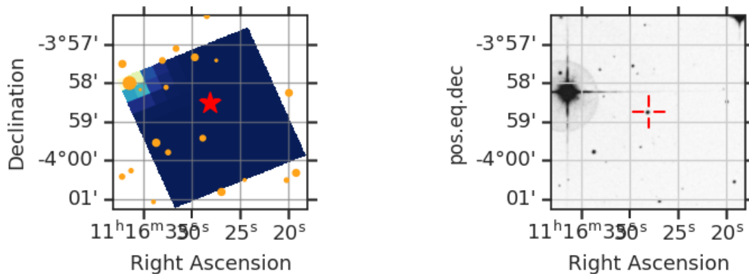
Fig 7. The locations of nearby GAIA DR2 stars with a magnitude difference less than 5 (orange circle) within the Tess Cut Out around TIC 443616612 (red star). Only shown for one sector. Right: SDSS image of the surrounding field.
