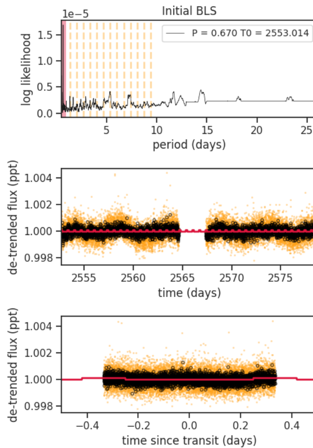
Fig 11. Box Least Square fitting (BLS) for whole lightcurve binned to 10 minutes. Top panel: log likelihood periodogram. The solid red line indicates the peak period and the dashed orange lines show the integer harmonics of this period. Middle panel: Full light curve, unbinned (orange) and binned to 10 minutes (black). The peak period is highlighted by the solid red lines. Bottom panel: Phase folded light curve where the found transit-event is fit with a simple box (red line).
