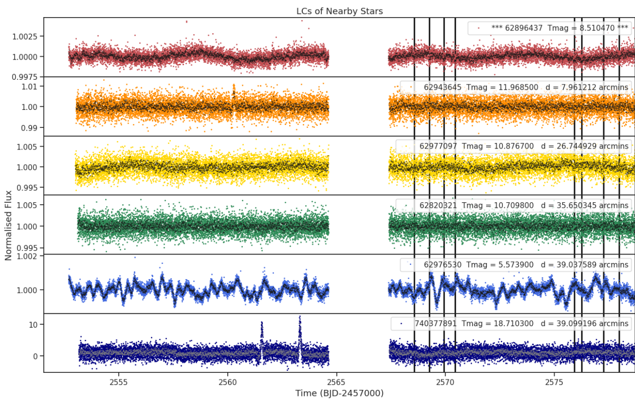
Fig 8. Lightcurves of the five closest stars to target 62896437 (top panel). The distances to the target star and the TESS magnitudes are shown for each star. Only ever shown for one sector.
