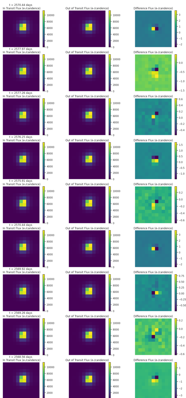
Fig 6. Difference images for target TIC 62896437 for each transit like event. Left: mean in-transit flux(left). Middle: mean out-of-transit flux. Right: difference between the mean out-of-transit and mean in-transit flux. Ensure that the change in brightness occurs on target.
