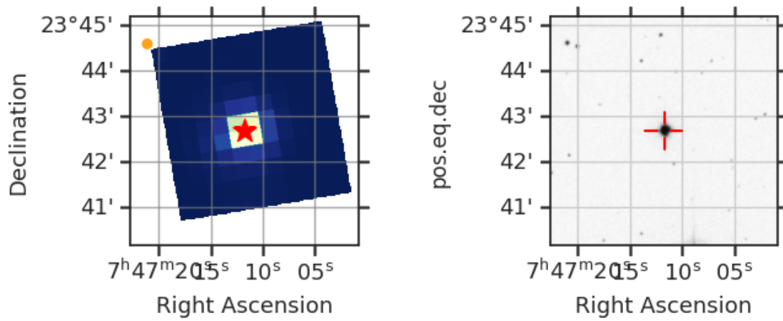
Fig 7. The locations of nearby GAIA DR2 stars with a magnitude difference less than 5 (orange circle) within the Tess Cut Out around TIC 62896437 (red star). Only shown for one sector. Right: SDSS image of the surrounding field.
