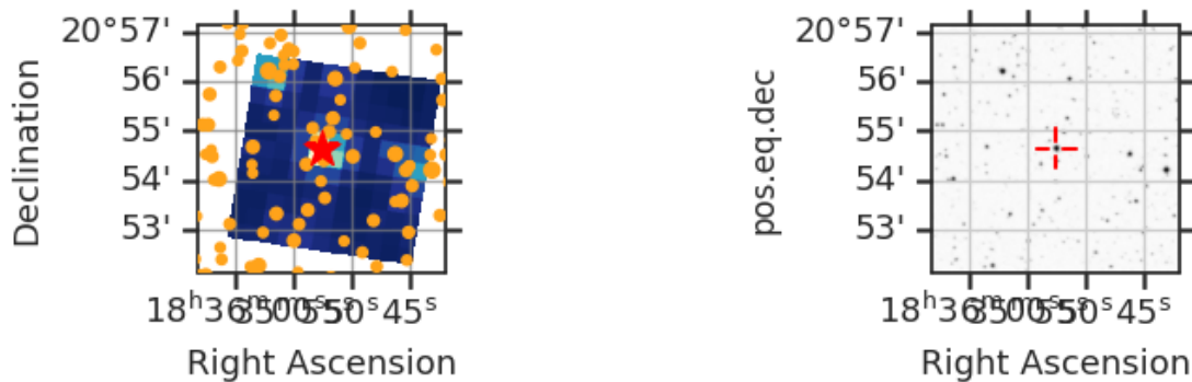
Fig 7. The locations of nearby GAIA DR2 stars with a magnitude difference less than 5 (orange circle) within the Tess Cut Out around TIC 8267970 (red star). Only shown for one sector. Right: SDSS image of the surrounding field.
