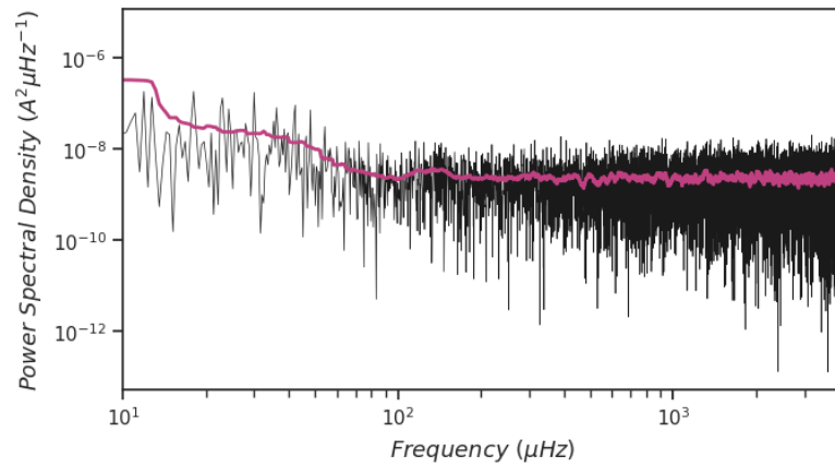
Fig 11. Lomb scargle power spectrum of the TESS lightcurve (black line) and a boxcar-smoothed periogram (pink line) computed with a window length of 20 micro Hz.
