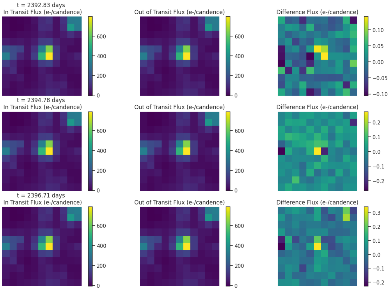
Fig 6. Difference images for target TIC 8267970 for each transit like event. Left: mean in-transit flux(left). Middle: mean out-of-transit flux. Right: difference between the mean out-of-transit and mean in-transit flux. Ensure that the change in brightness occurs on target.
