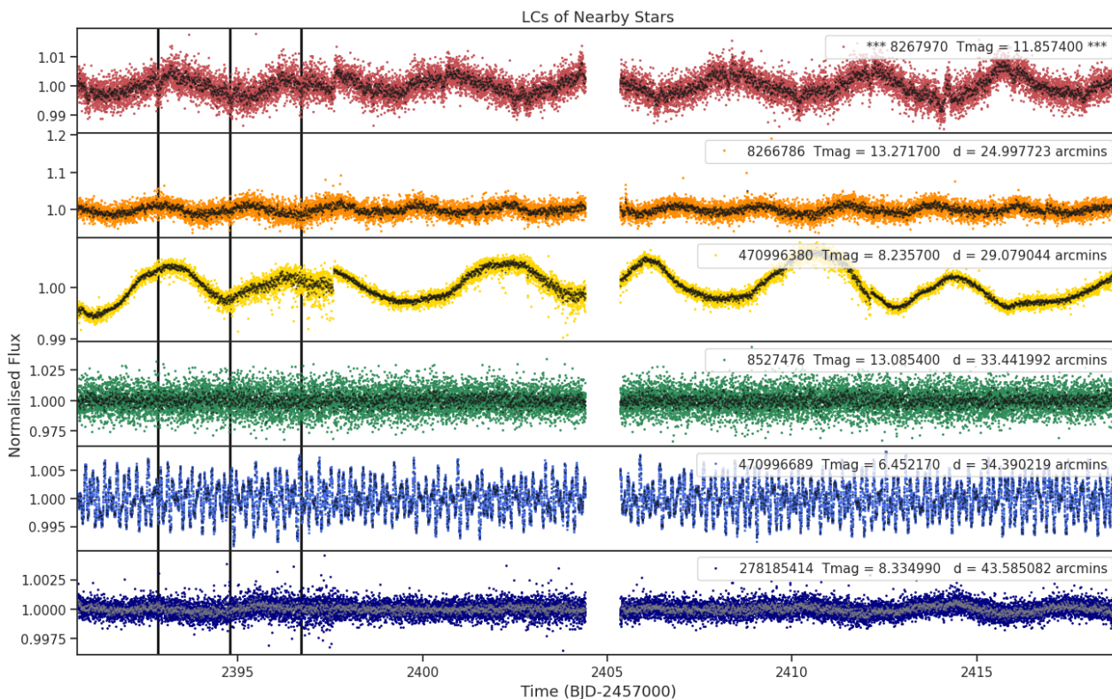
Fig 8. Lightcurves of the five closest stars to target 8267970 (top pannel). The distances to the target star and the TESS magnitudes are shown for each star. Only ever shown for one sector.
