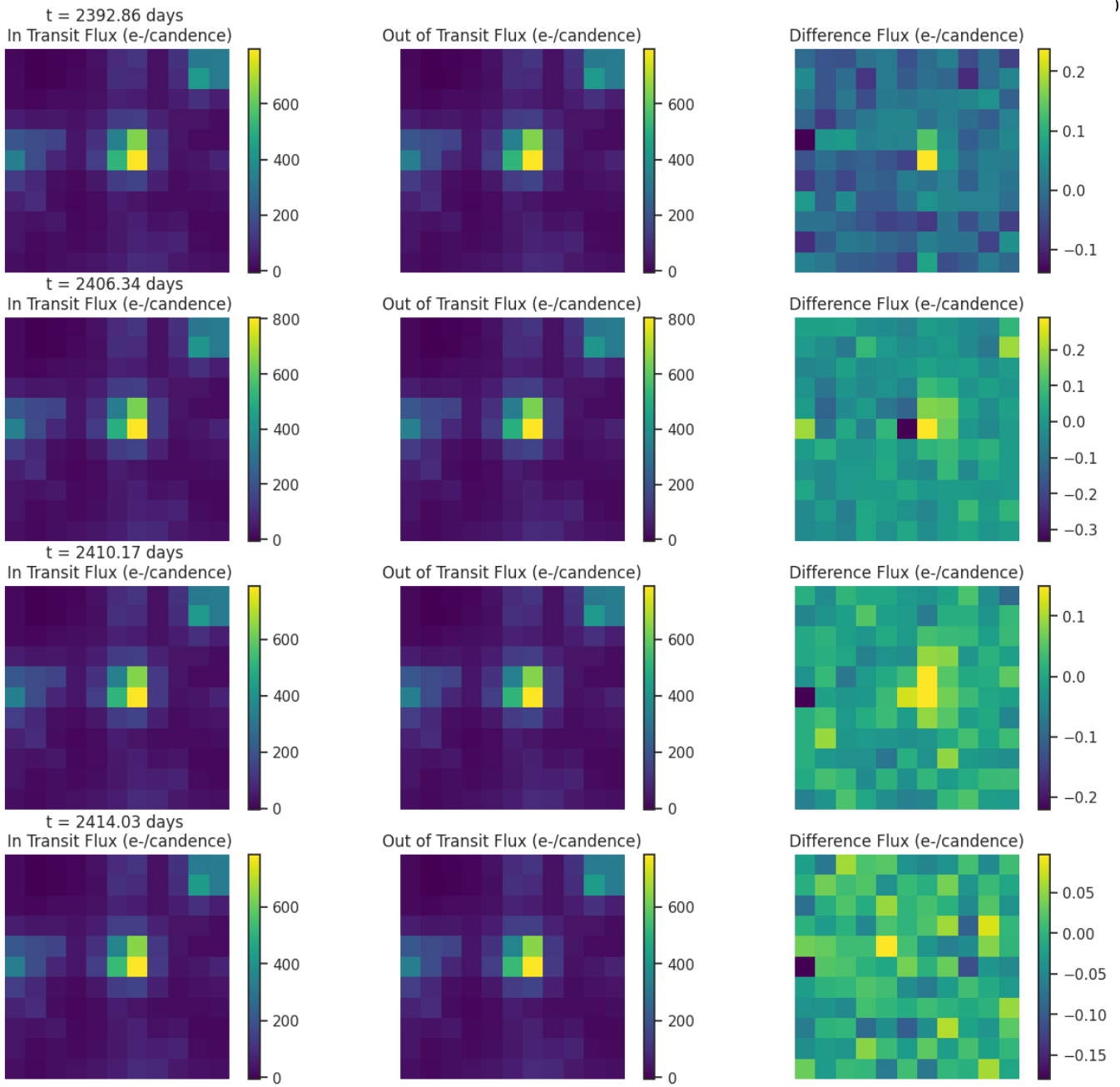
Fig 6. Difference images for target TIC 8267970 for each transit like event. Left: mean in-transit flux(left). Middle: mean out-of-transit flux. Right: difference between the mean out-of-transit and mean in-transit flux. Ensure that the change in brightness occurs on target.
