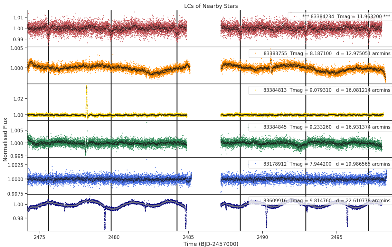
Fig 8. Lightcurves of the five closest stars to target 83384234 (top pannel). The distances to the target star and the TESS magnitudes are shown for each star. Only ever shown for one sector.
