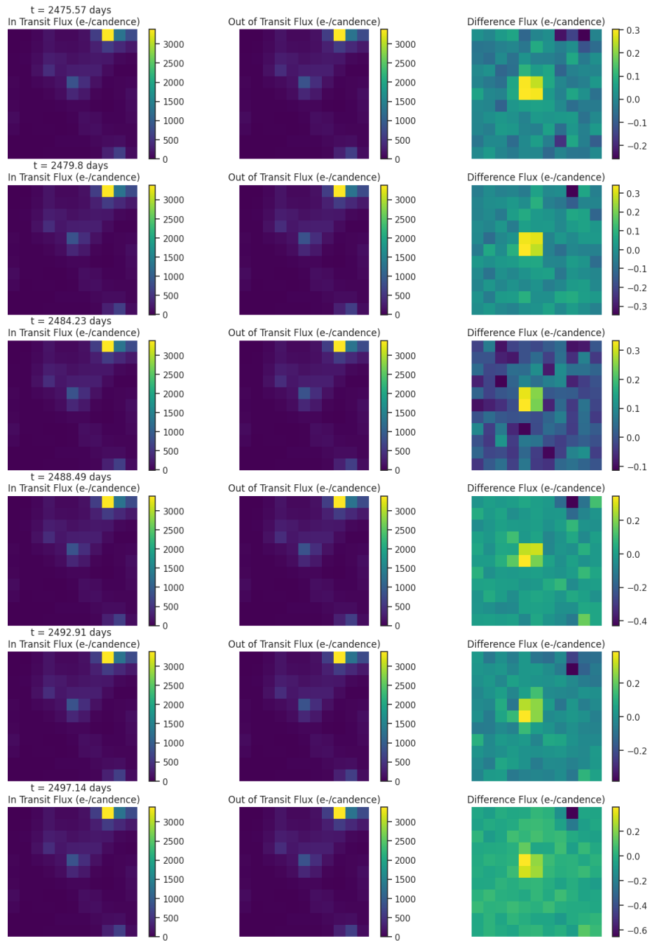
Fig 6. Difference images for target TIC 83384234 for each transit like event. Left: mean in-transit flux(left). Middle: mean out-of-transit flux. Right: difference between the mean out-of-transit and mean in-transit flux. Ensure that the change in brightness occurs on target.
