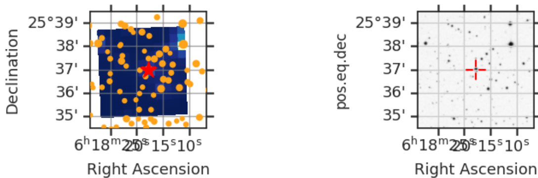
Fig 7. The locations of nearby GAIA DR2 stars with a magnitude difference less than 5 (orange circle) within the Tess Cut Out around TIC 83384234 (red star). Only shown for one sector. Right: SDSS image of the surrounding field.
