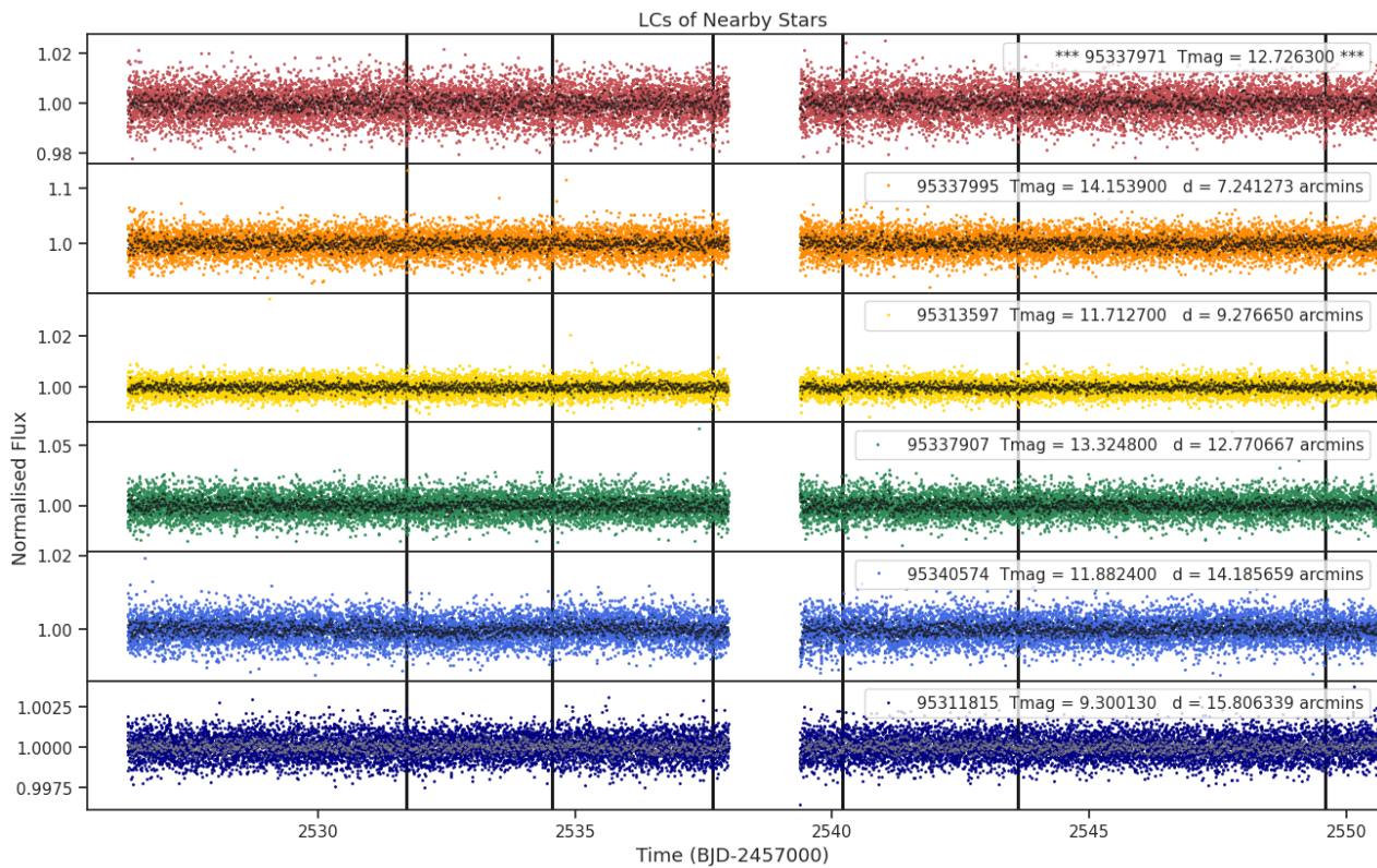
Fig 8. Lightcurves of the five closest stars to target 95337971 (top panel). The distances to the target star and the TESS magnitudes are shown for each star. Only ever shown for one sector.
