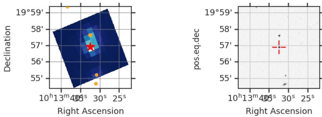
Fig 7. The locations of nearby GAIA DR2 stars with a magnitude difference less than 5 (orange circle) within the TESS Cut Out around TIC 95337971 (red star). Only shown for one sector. Right: SDSS image of the surrounding field.
