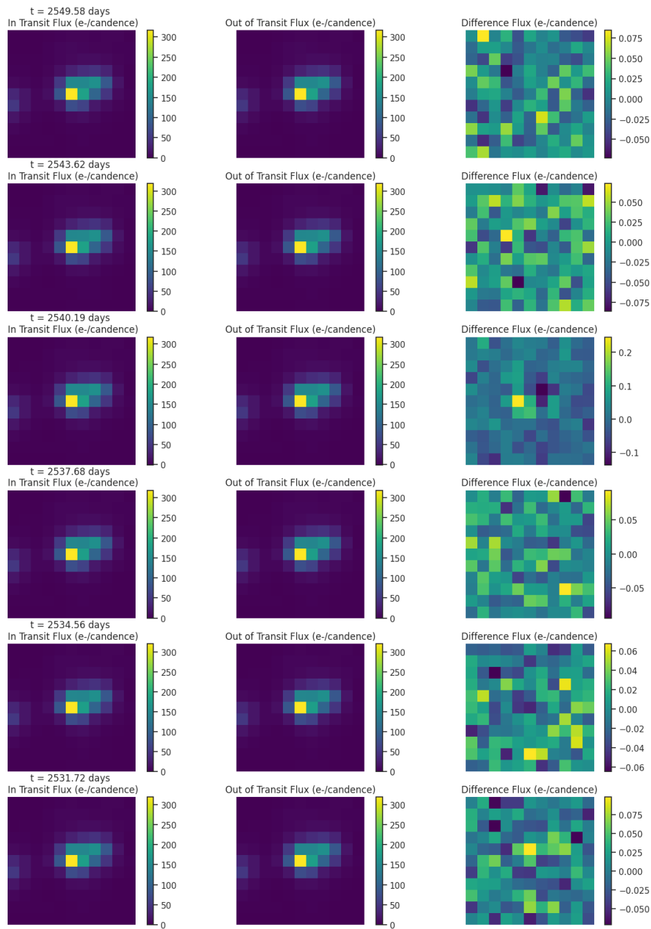
Fig 6. Difference images for target TIC 95337971 for each transit like event. Left: mean in-transit flux(left). Middle: mean out-of-transit flux. Right: difference between the mean out-of-transit and mean in-transit flux. Ensure that the change in brightness occurs on target.
