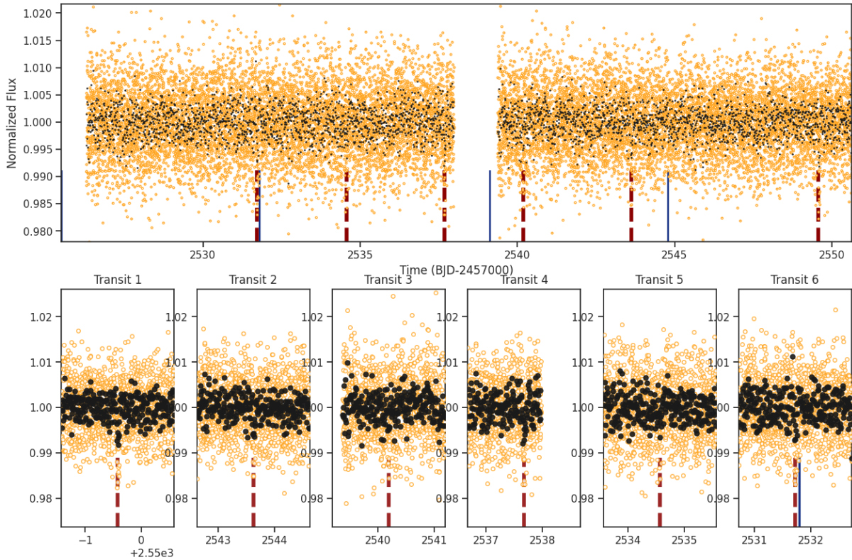
Fig 1. Full lightcurve for target TIC 95337971. The solid blue lines at the bottom of the figure indicated the times of the reaction wheel momentum dumps and the dashed black line(s) show the time(s) of the marked transit event(s). Momentum dumps occur around every 2 to 2.5 days and typically last around half an hour.
