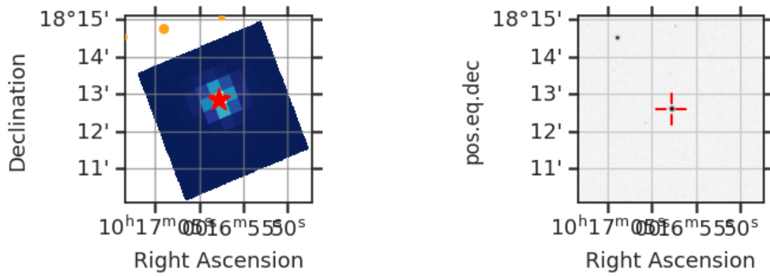
Fig 7. The locations of nearby GAIA DR2 stars with a magnitude difference less than 5 (orange circle) within the TESS Cut Out around TIC 95361530 (red star). Only shown for one sector. Right: SDSS image of the surrounding field.
