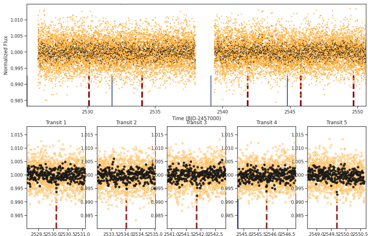
Fig 1. Full lightcurve for target TIC 95361530. The solid blue lines at the bottom of the figure indicated the times of the reaction wheel momentum dumps and the dashed black line(s) show the time(s) of the marked transit event(s). Momentum dumps occur around every 2 to 2.5 days and typically last around half an hour.
