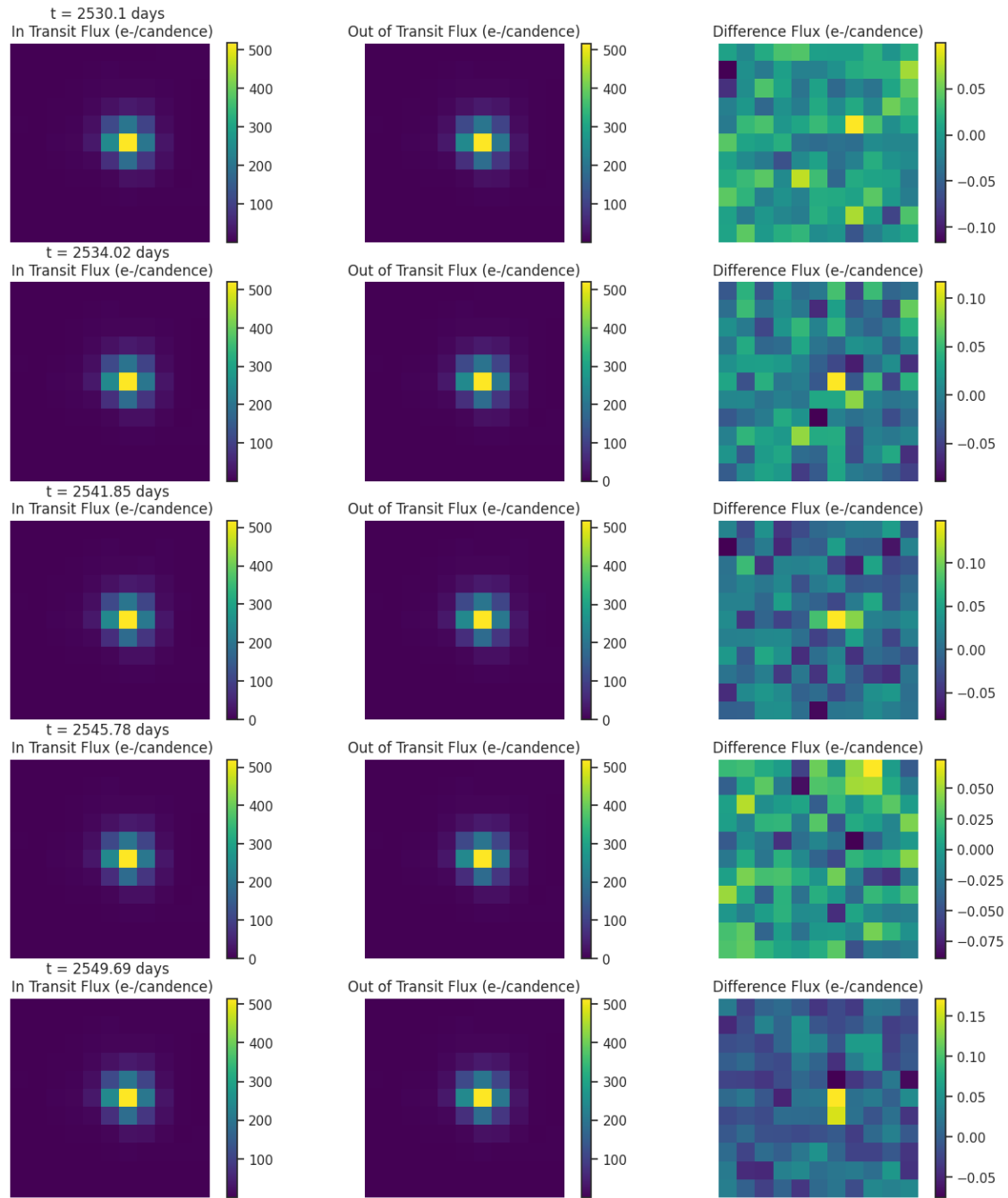
Fig 6. Difference images for target TIC 95361530 for each transit like event. Left: mean in-transit flux(left). Middle: mean out-of-transit flux. Right: difference between the mean out-of-transit and mean in-transit flux. Ensure that the change in brightness occurs on target.
