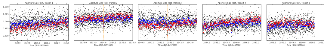
Fig 4. The lightcurve around the time of each transit-like event extracted with the SPOC pipeline defined aperture (binned:blue, uninned:grey) and the with an aperture that is 40 per cent smaller (red). The flux is extracted from the target pixel files (TPFs) and has not been detrended or corrected for systematics. The vertical orange line indicates the time of the transit-like event.
