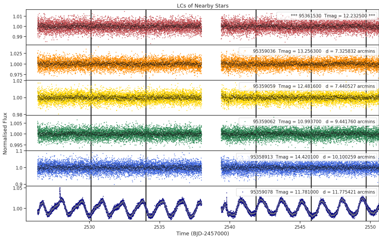
Fig 8. Lightcurves of the five closest stars to target 95361530 (top pannel). The distances to the target star and the TESS magnitudes are shown for each star. Only ever shown for one sector.
